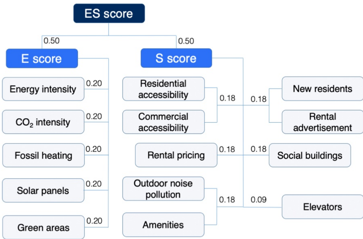
Figure 34: Indicator weights
